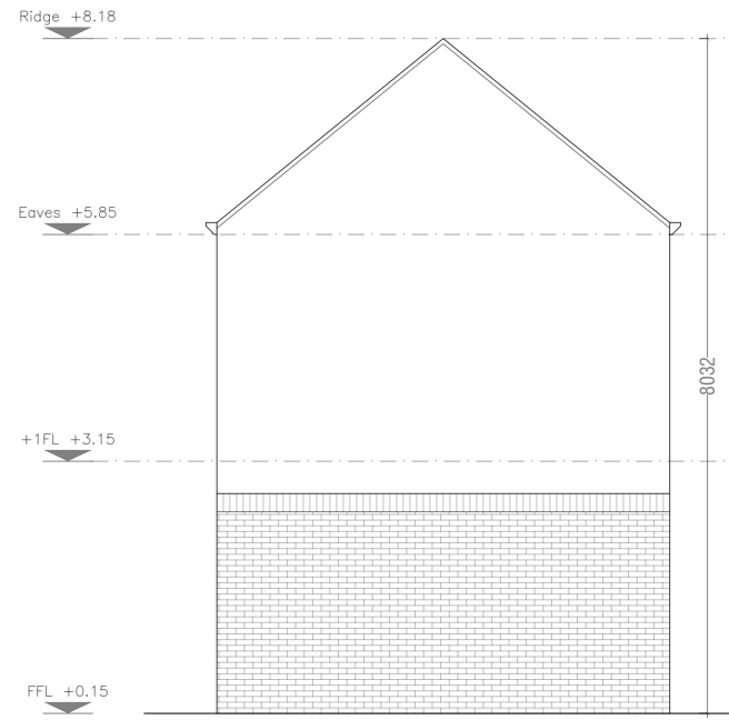
House Type O1/O2 Semi-Detached/End of Terrace Side Elevation
