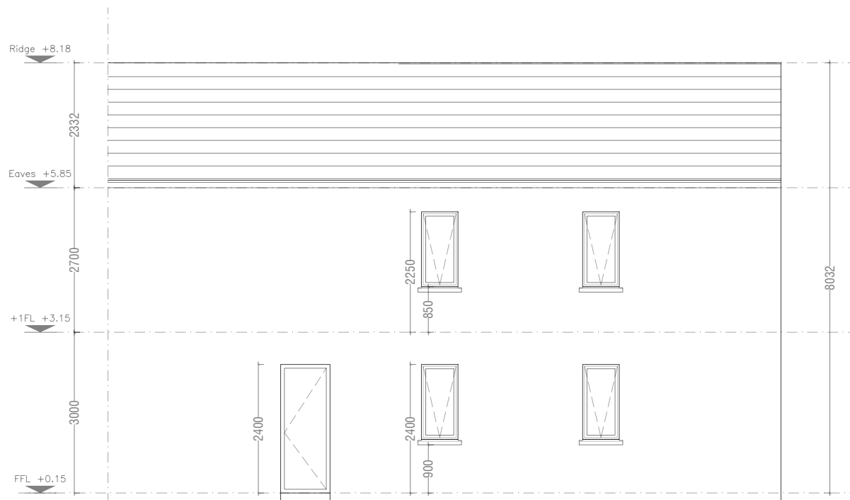
House Type O1/O2 Semi-Detached/End of Terrace Rear Elevation
